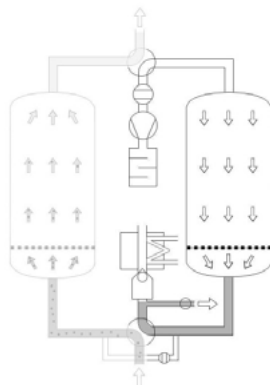
Fáza expanzie
